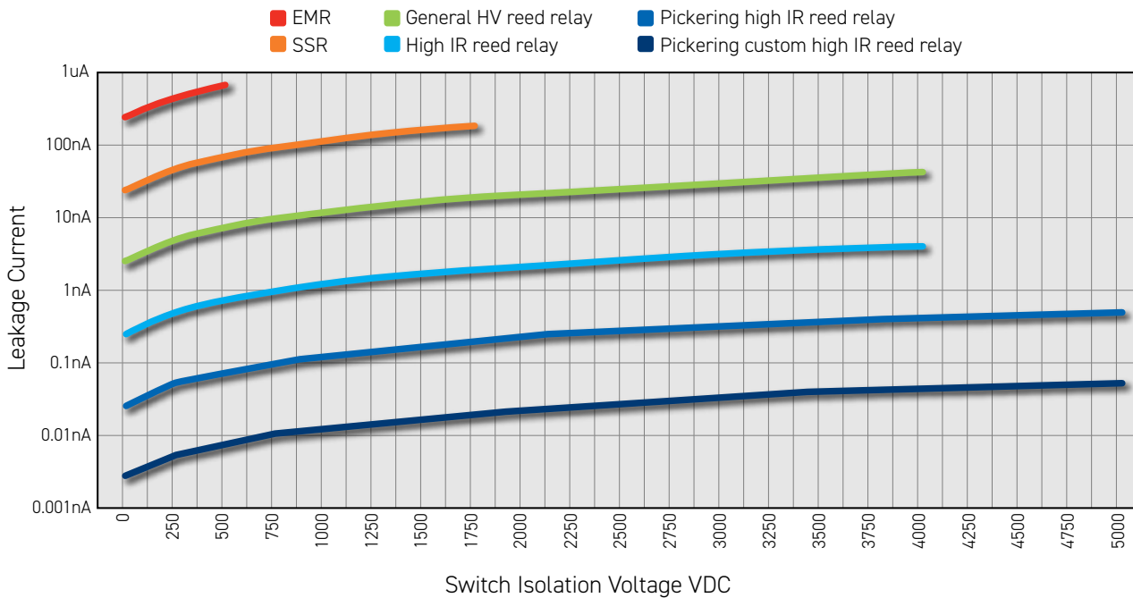
Typical Leakage Current vs Voltage
